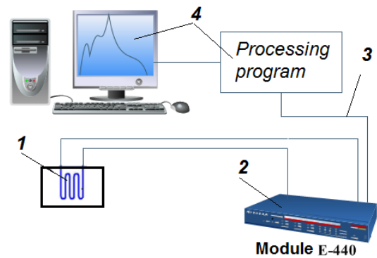
Figure 8. Installation for the acquisition of the force acting on press slide
